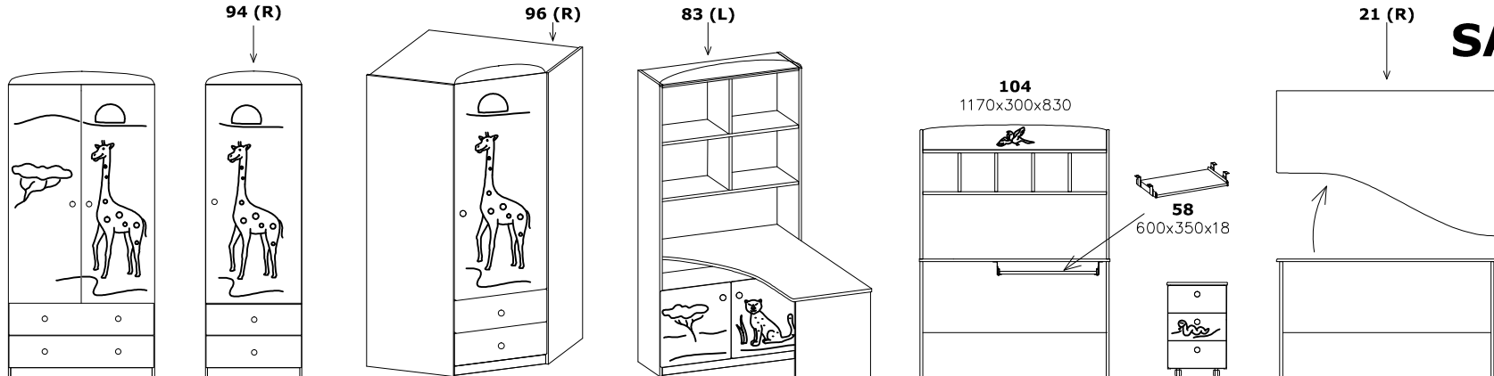
93 895x566x1800(+100) 94 (R) 595x566x1800(+100) 96 (R) 985x985x1800(+100) 83 (L) 895(510)x1320x1800(+100) 104 1170x300x830 47 1200x540x730 46 380x450x600 21 (R) 1300x900(510)x730 95 (L) 97 (L) 82 (R) 83 (L) 58 600x350x18 21 (L)
