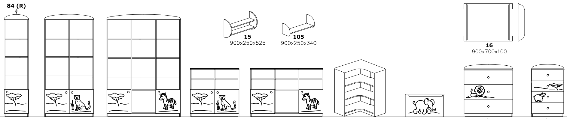
84 (R) 456x340x1800(+100) 86 895x340x1800(+100) 87 1332x340x1800(+100) 88 900x345x890 89 1338x345x890 45 800x800x890 17 700x395x420 1 900x450x890(+100) 2 600x450x890(+100) 85 (L) 15 900x250x525 105 900x250x340 16 900x700x100
